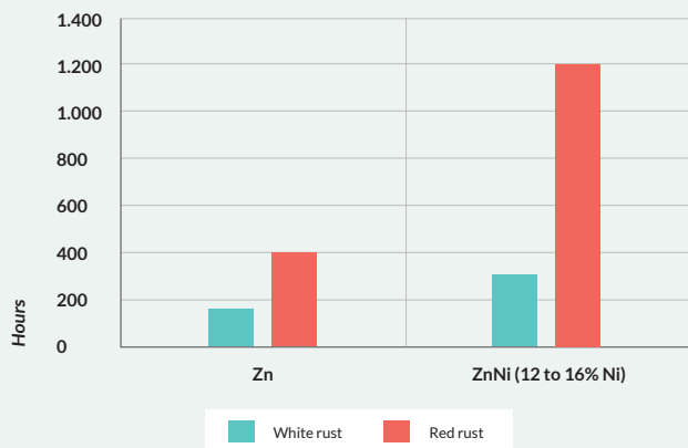
Comparing ZnNi and Zn coatings on corrosion resistance (Neutral Salt Spray (ASTM B117))
